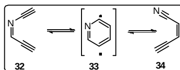
Scheme 6: Aza-Bergman Cyclization
